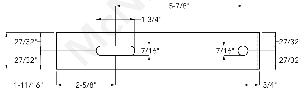
End View
