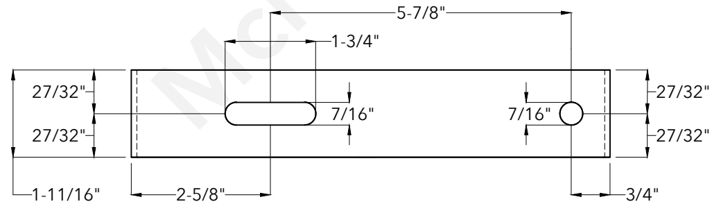
End View
