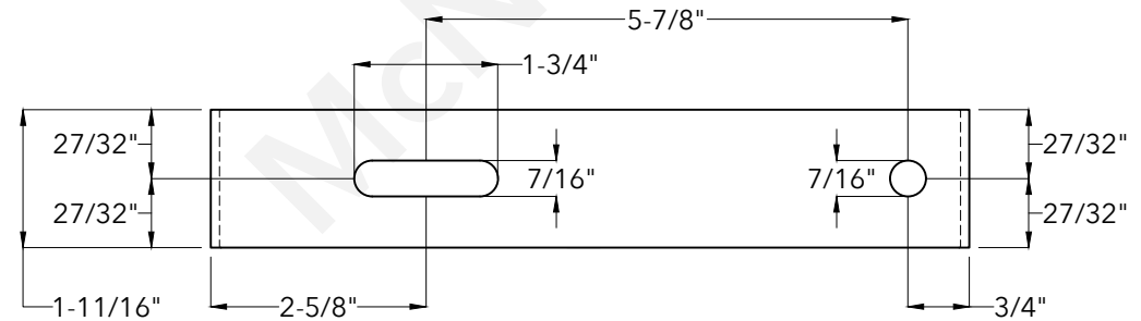
End View
