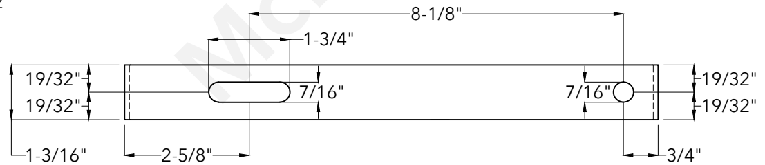
End View
