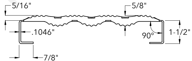
END VIEW
