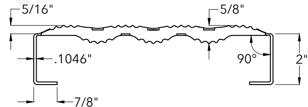
END VIEW
