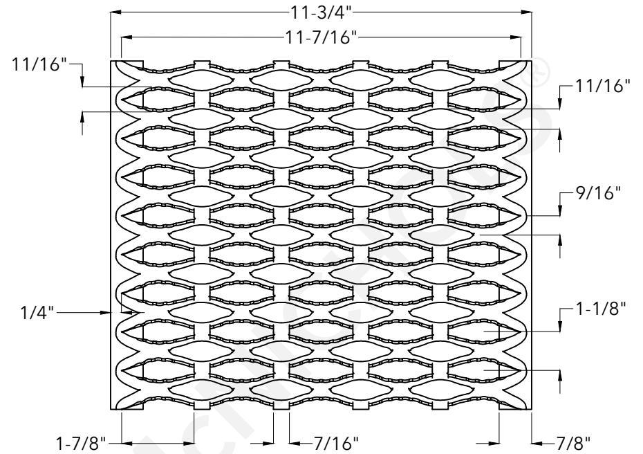
END VIEW
