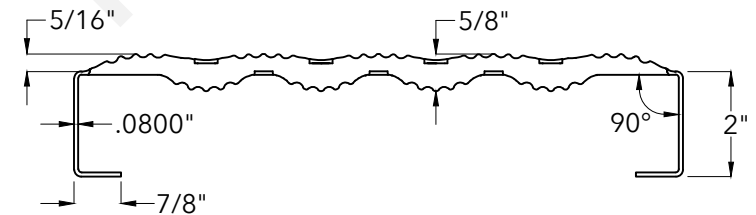
END VIEW
