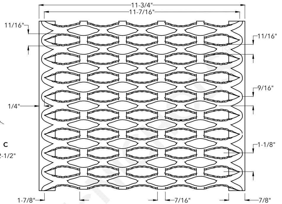
End View
