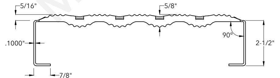
End View
