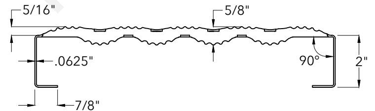
END VIEW
