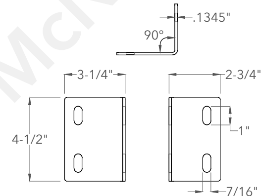
Mounting Bracket
