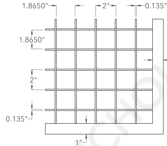
Mounting Bracket
