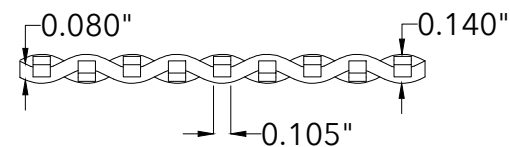
End View
