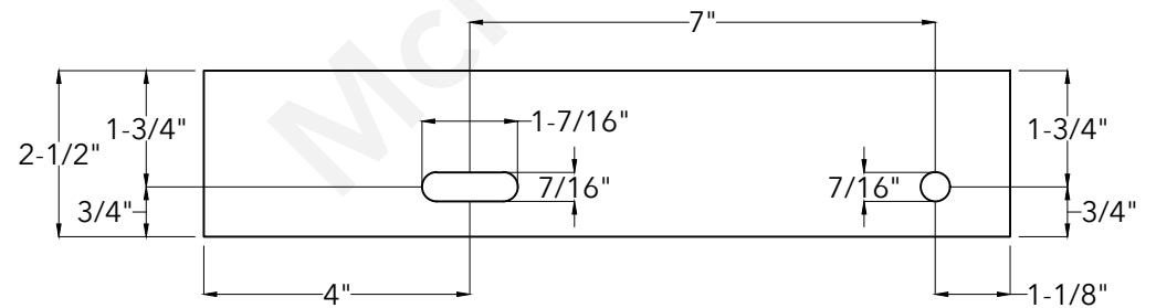
End View
