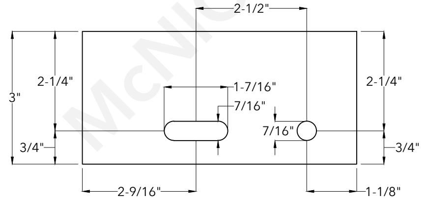
End View
