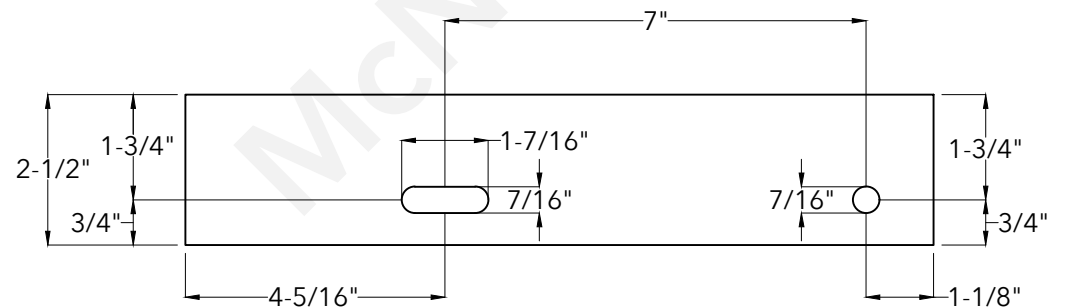
End View
