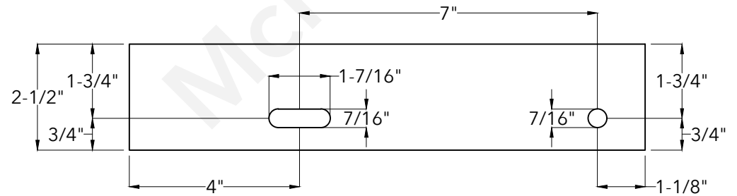
End View
