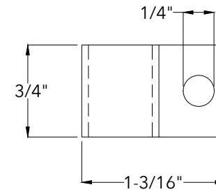
Clip Top View
