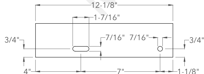
Side View
