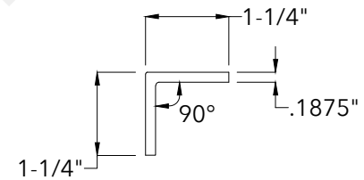
End View
