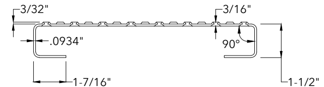
End View
