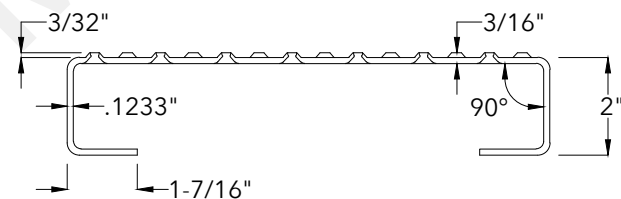
End View
