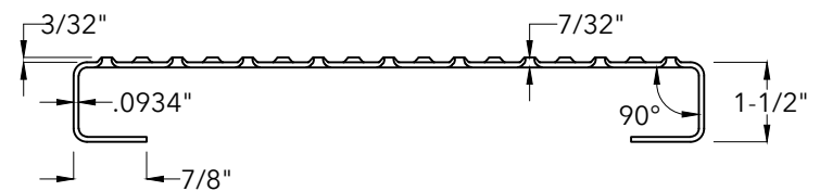
End View
