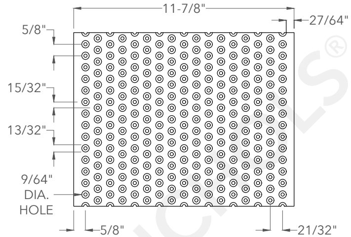
End View
