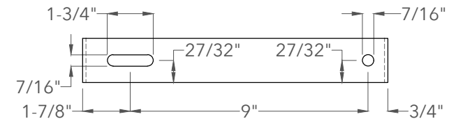
End View
