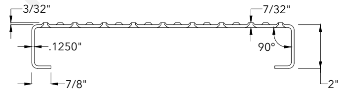
End View
