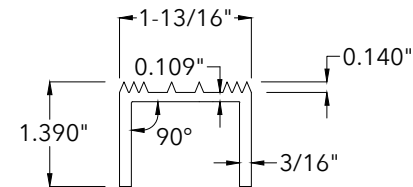
End View
