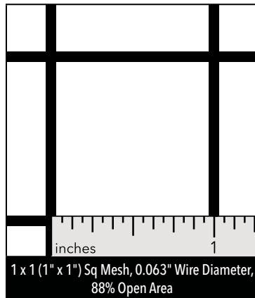
SQUARE MESH
